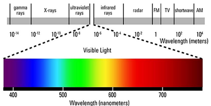
Fig. 4.1 Electromagnetic spectrum
