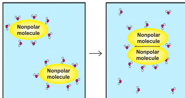
Fig. 2.6: Hydrophobic exclusion
