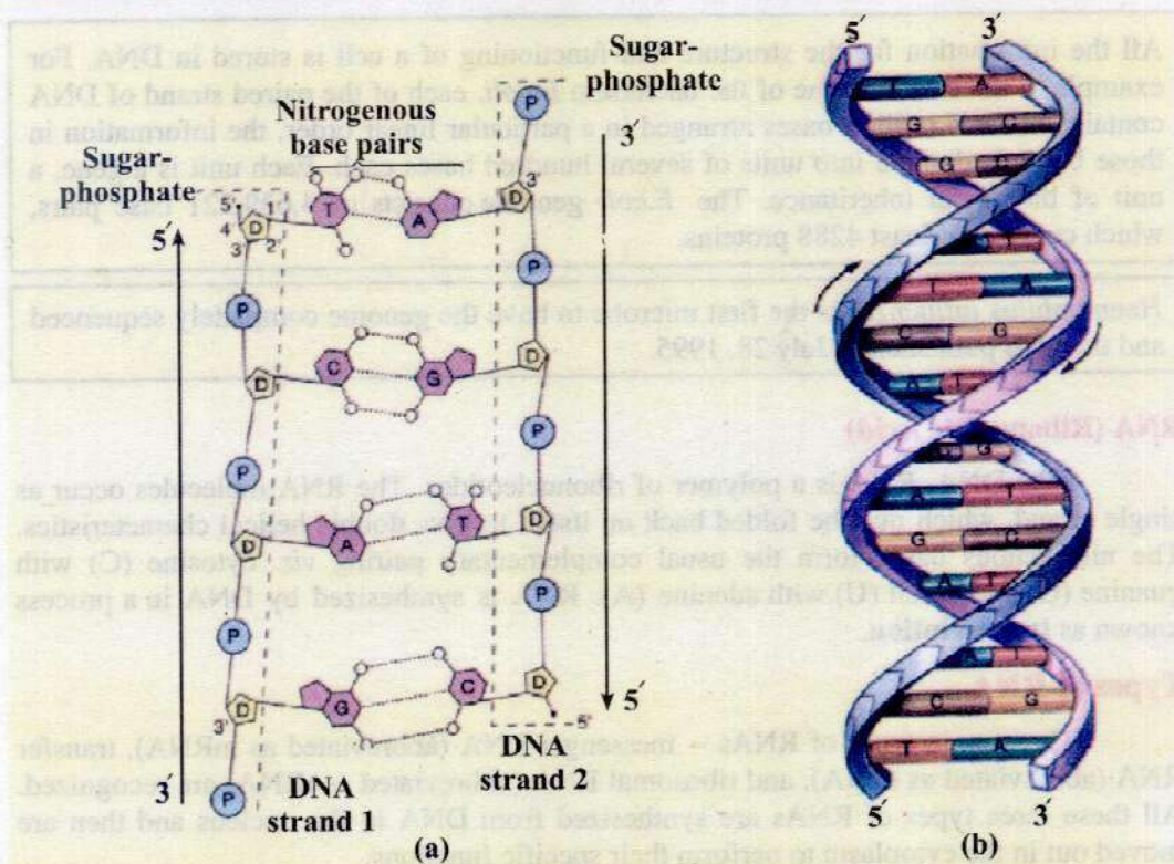
Fig. 2.15 Model of DNA. Double helical structure of DNA proposed by Watson & Crick (b). A hypothetical sequence of nucleotides (on the left side) shows hydrogen bonding between the complementary bases. Note a double bond between A and T, and triple bond between C and G (a).
