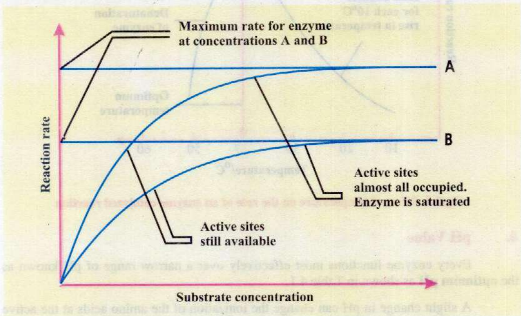
Fig. 3.4. Effect of substrate concentration on the rate of an enzyme catalyzed reaction.
