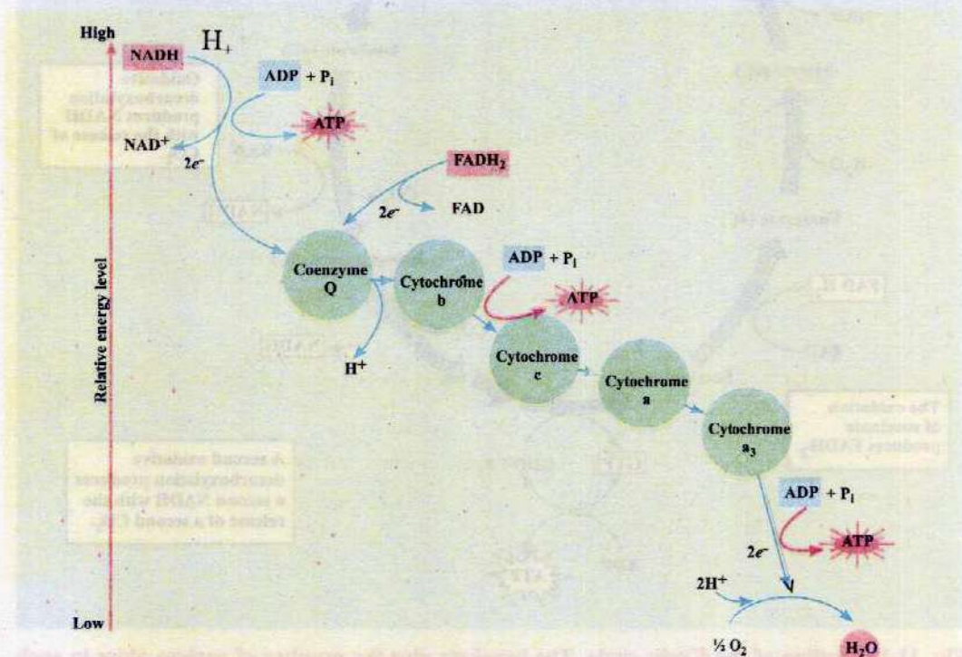
Fig. 11.14 The respiratory electron transport chain and its coupling with oxidative phosphorylation.
