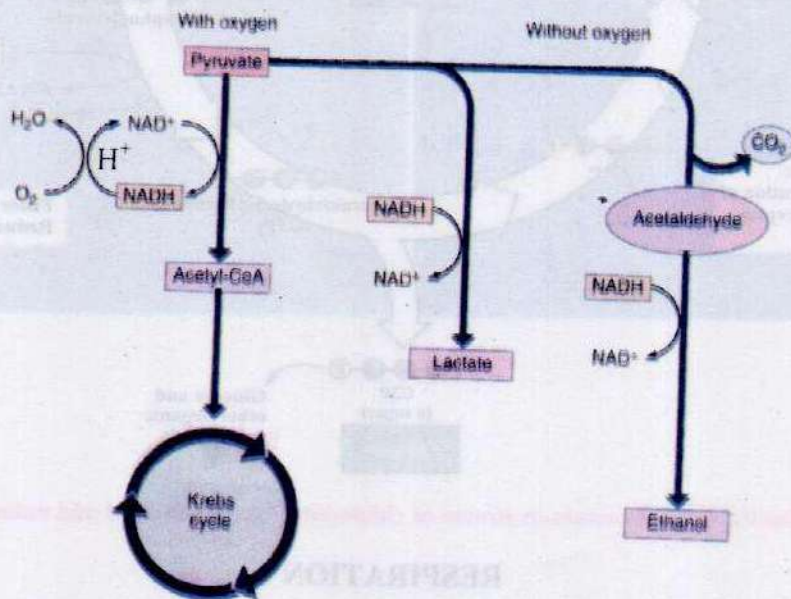
Fig. 11.11 Pyruvate, the end product of glycolysis, follows different catabolic pathways depending on the organism and the metabolic condition.
