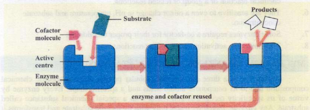
Fig. 3.1 Substrate molecules will not fit correctly at the active centre and there will be no catalytic action unless the cofactor molecule is also present.
