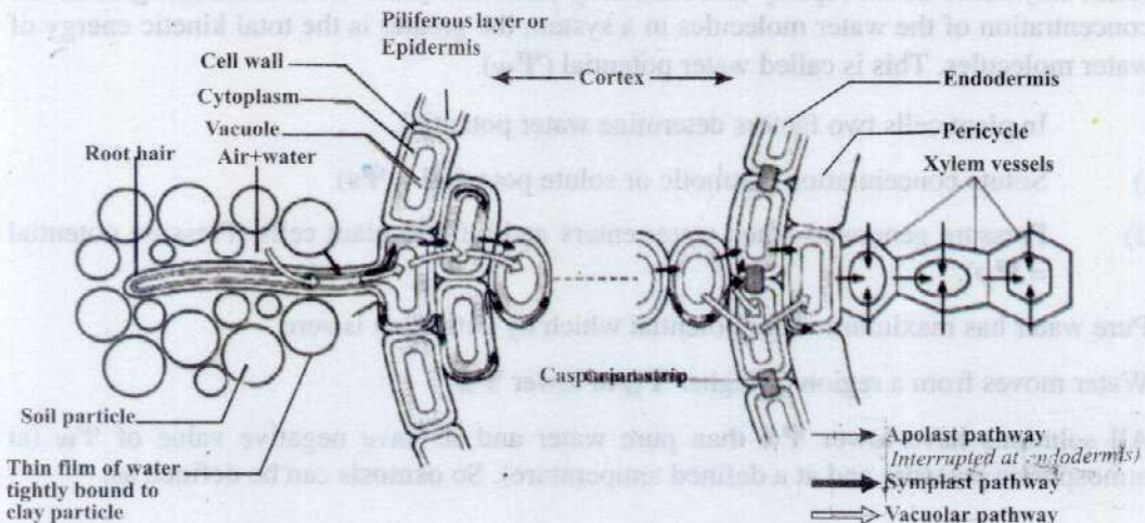
Fig. 14.2 Diagrammatic representation of water and ion movement across a root showing transverse section. The apoplast pathway is of greatest importance for both water and solutes. The symplast pathway is less important, except for salts in the region of the endodermis. Movement along the vacuolar pathway is negligible.
