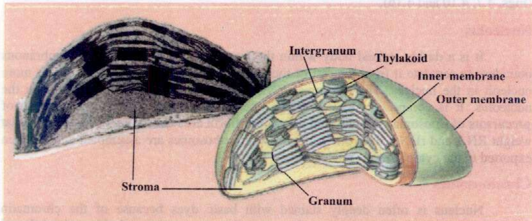
Fig. 4.14. : Diagram of chloroplast showing the main structural components.
