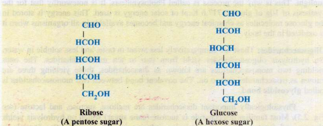
Fig. 2.3 Structure of Ribose and Glucose.
