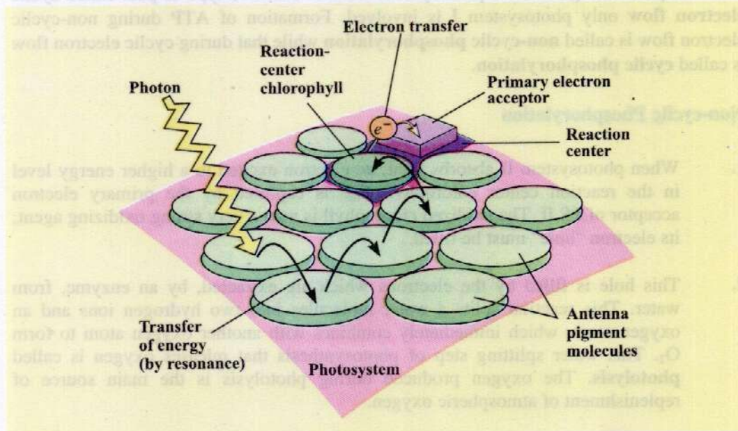
Fig. 11.6: Light harvesting photosystem. Energy of light (photon) absorbed by photosynthetic pigment molecules is transferred from molecule to molecule, and finally reaches the reaction centre where actual energy conversion begins.
