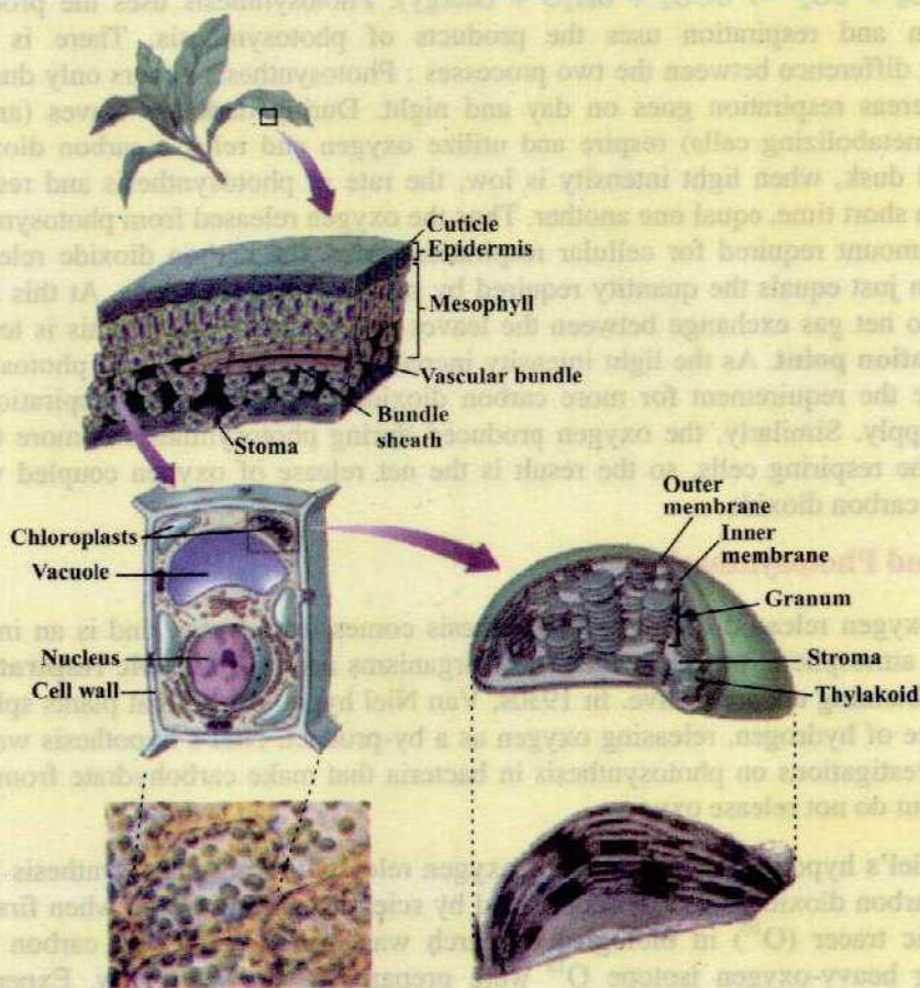
Fig. 11.1 A plant possesses thick layer of mesophyll cells rich in chloroplasts. Thylakoids in chloroplasts are stacked into grana. Light reactions take place on the grana, and dark reactions in the stroma.
