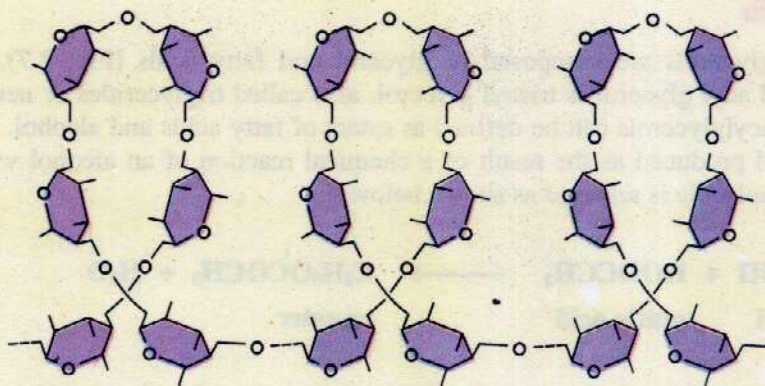
Fig 2.6 : Polysaccharides are polymers of monosaccharides.
