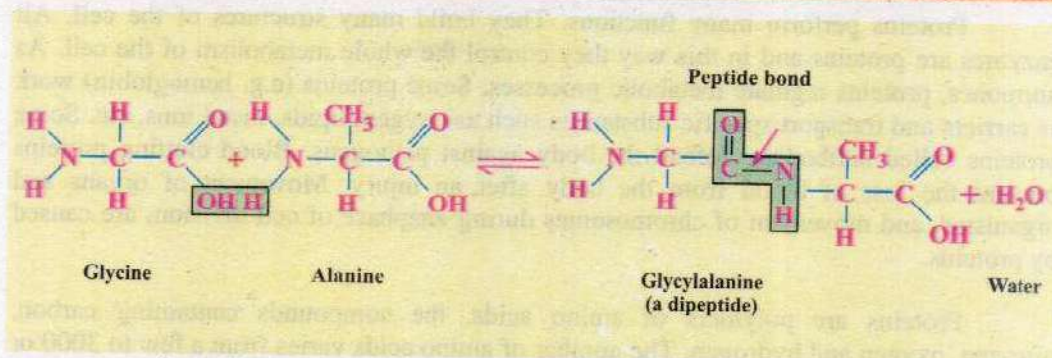
Fig. 2.10 Peptide linkage – formation of peptide bond
